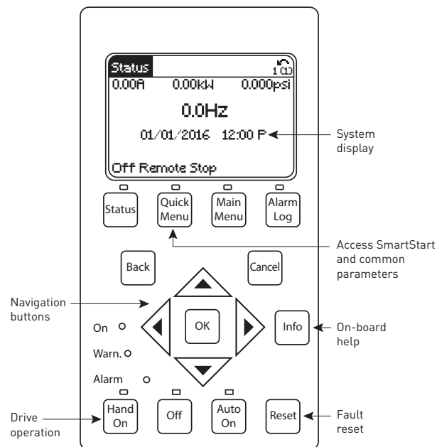
Figure 1. Local Control Panel — Your interface to the drive.
