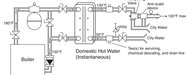
Diagram 3-Instantaneous
