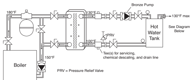
Diagram 1-Recirc to Tank
