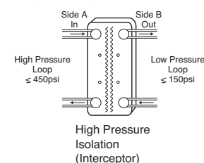
Diagram 3-High Pressure Isolation
