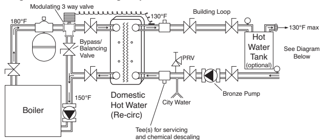
Diagram 3-Instantaneous
