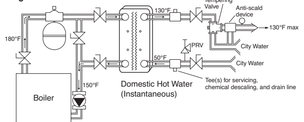
Diagram 3-Instantaneous
